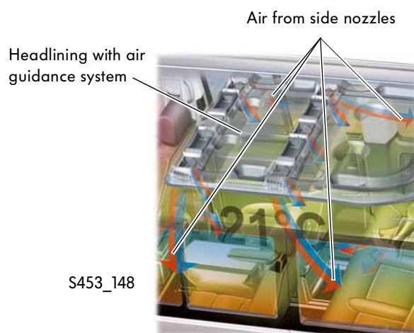
Nozzles in headlining - for air-conditioning the compartment air
